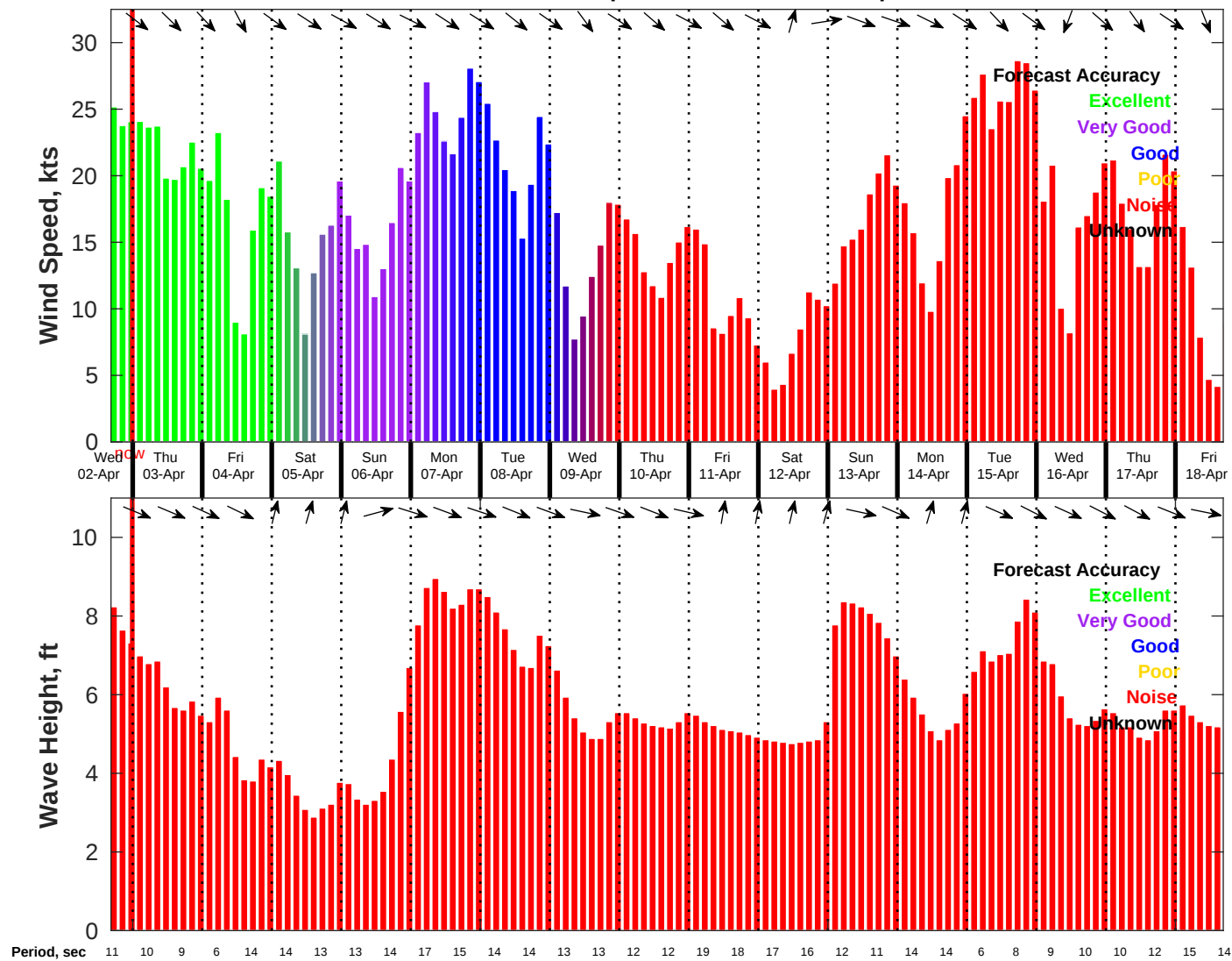
Wind & Wave Forecast for NDBC 46069 from 02-Apr-2025 16:00:00 to 18-Apr-2025 16:00:00
