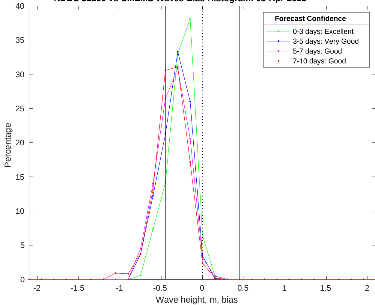
NDBC 51209 vs CMEMS Waves Bias Histogram: 03-Apr-2025
