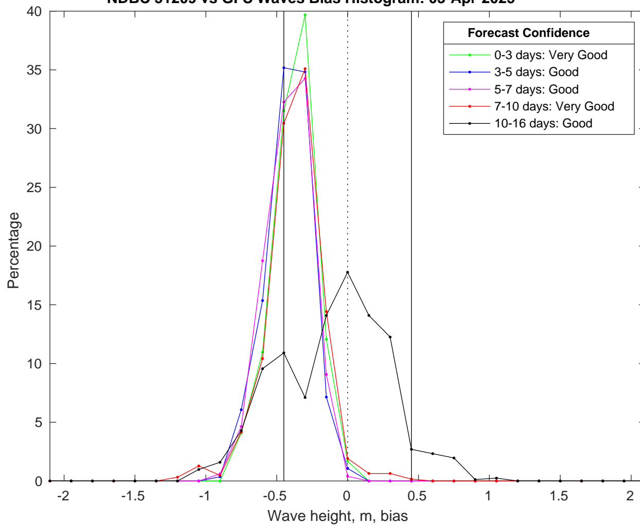
NDBC 51209 vs GFS Waves Bias Histogram: 03-Apr-2025
