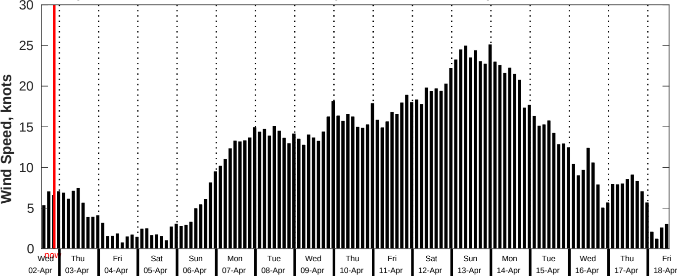
GFS Wind Speed Forecast for NDBC 51209 from 02-Apr-2025 13:00:00 to 18-Apr-2025 13:00:00
