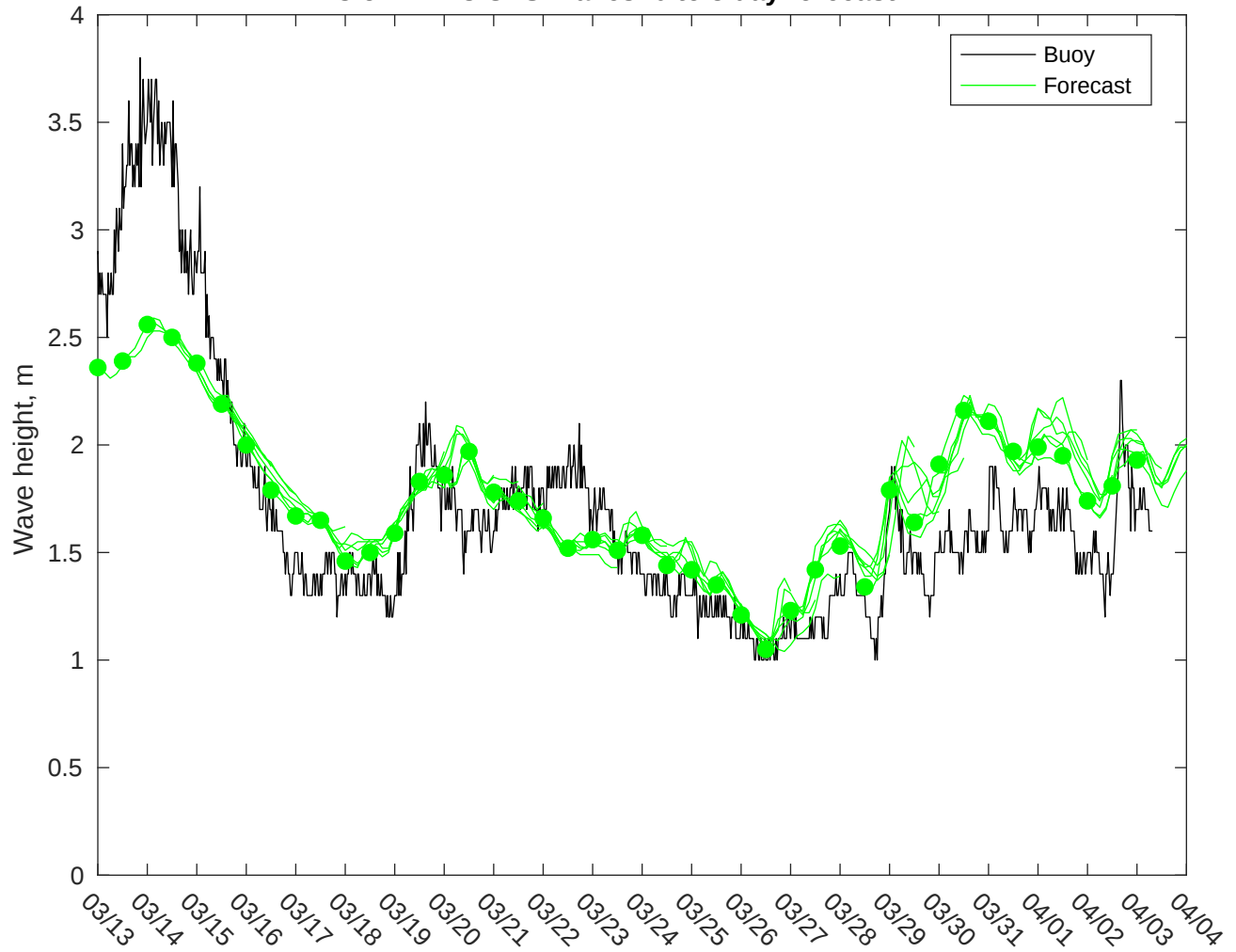
NDBC 52211 vs GFS Waves: 0 to 3 day forecast
