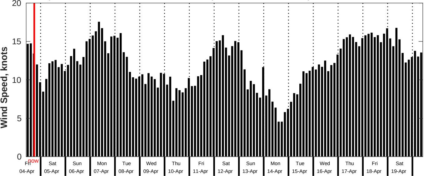
GFS Wind Speed Forecast for NDBC 52211 from 03-Apr-2025 10:00:00 to 19-Apr-2025 10:00:00
