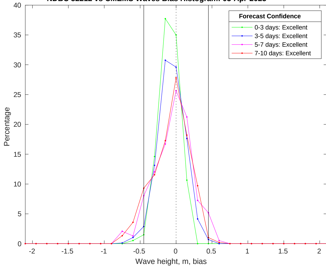
NDBC 52212 vs CMEMS Waves Bias Histogram: 03-Apr-2025
