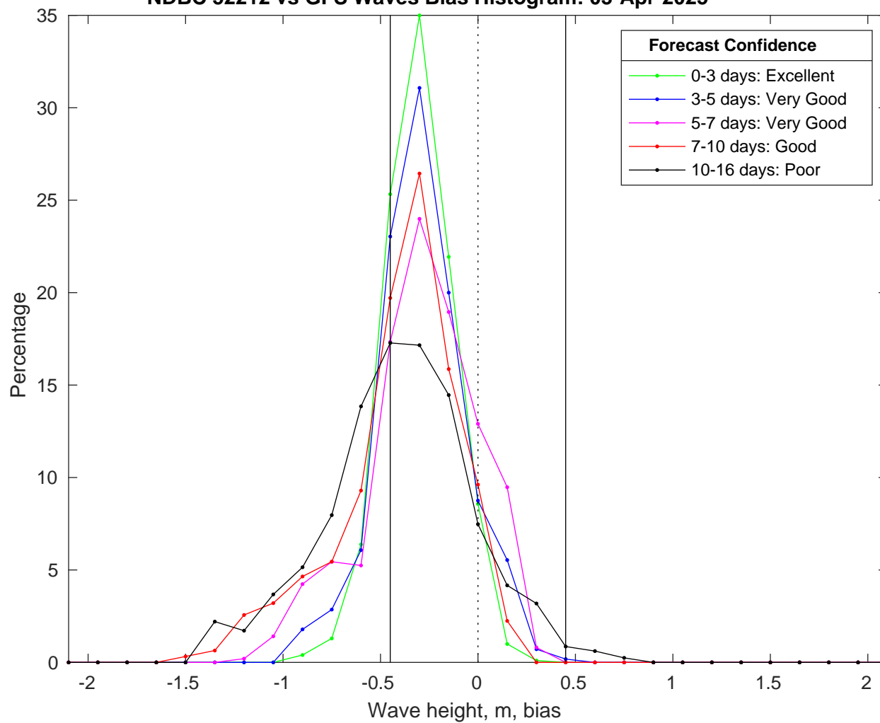
NDBC 52212 vs GFS Waves Bias Histogram: 03-Apr-2025
