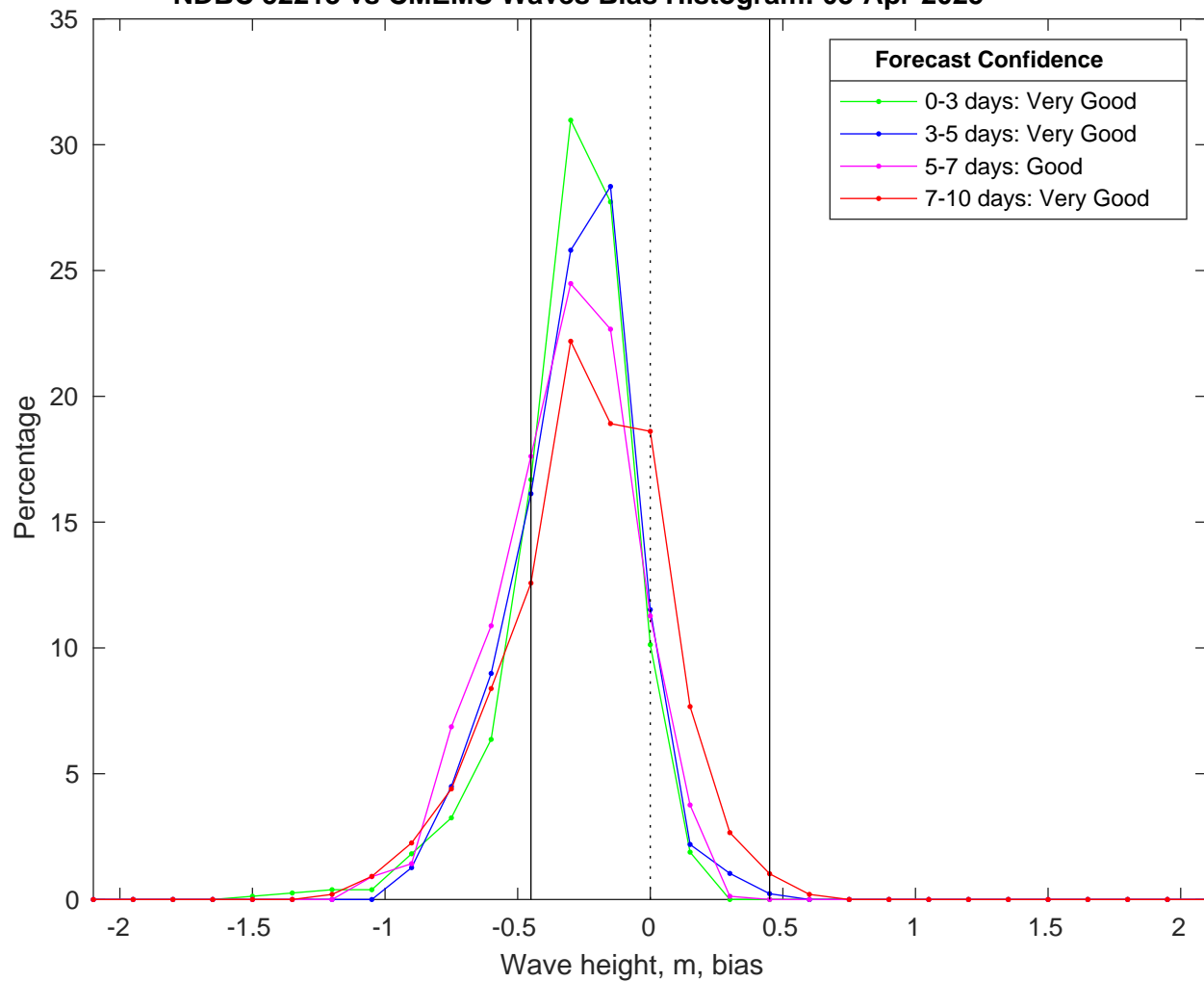
NDBC 52213 vs CMEMS Waves Bias Histogram: 03-Apr-2025
