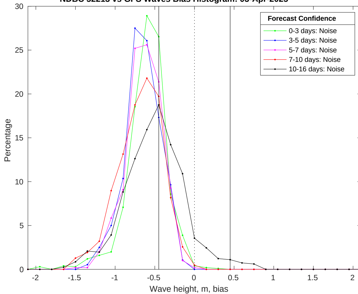
NDBC 52213 vs GFS Waves Bias Histogram: 03-Apr-2025
