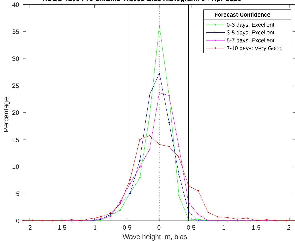
NDBC 41004 vs CMEMS Waves Bias Histogram: 04-Apr-2025
