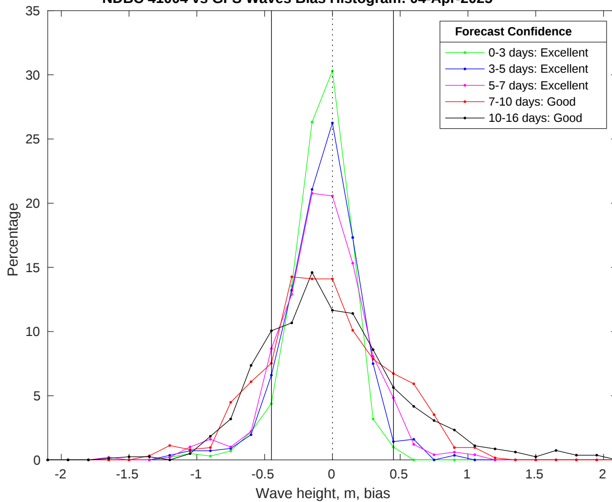
NDBC 41004 vs GFS Waves Bias Histogram: 04-Apr-2025
