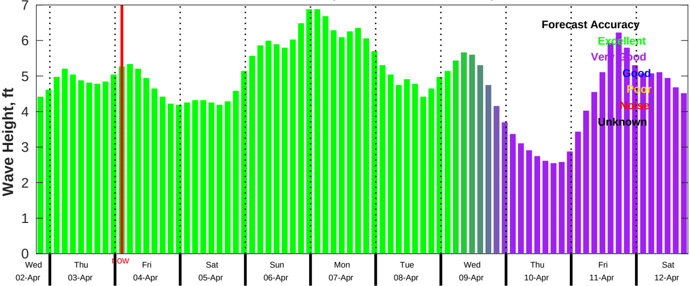
CMEMS Wave Forecast for NDBC 41004 from 02-Apr-2025 19:00:00 to 12-Apr-2025 19:00:00
