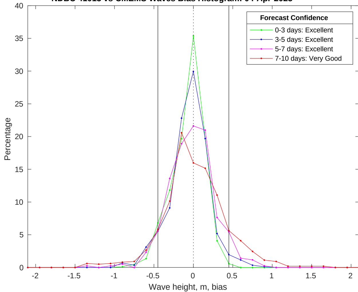
NDBC 41013 vs CMEMS Waves Bias Histogram: 04-Apr-2025
