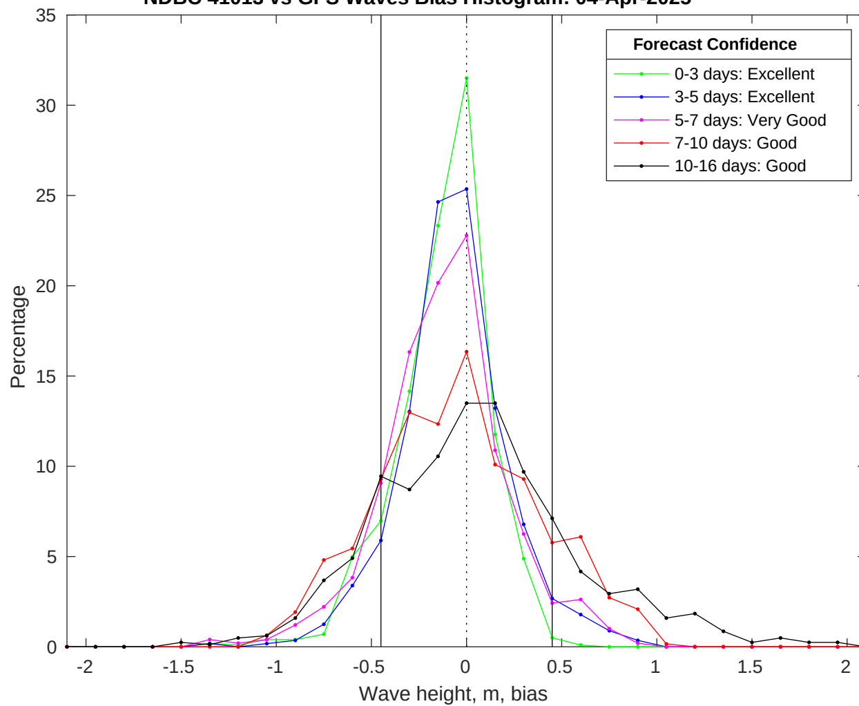
NDBC 41013 vs GFS Waves Bias Histogram: 04-Apr-2025
