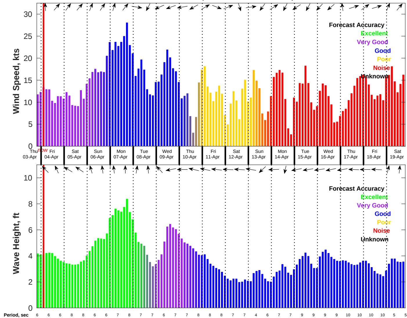
Wind & Wave Forecast for NDBC 41013 from 03-Apr-2025 19:00:00 to 19-Apr-2025 19:00:00
