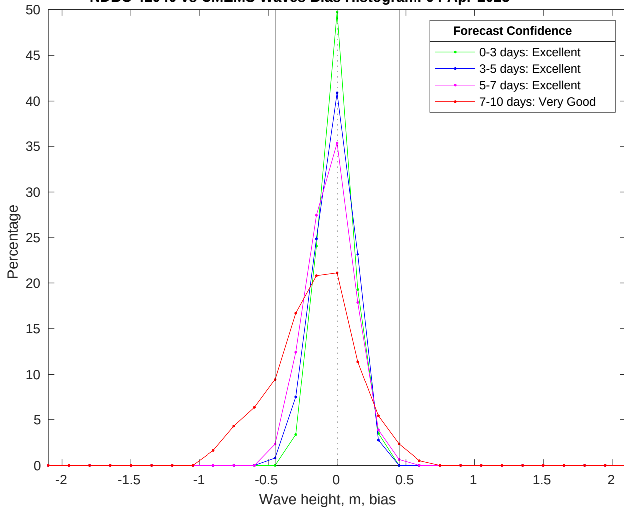
NDBC 41040 vs CMEMS Waves Bias Histogram: 04-Apr-2025
