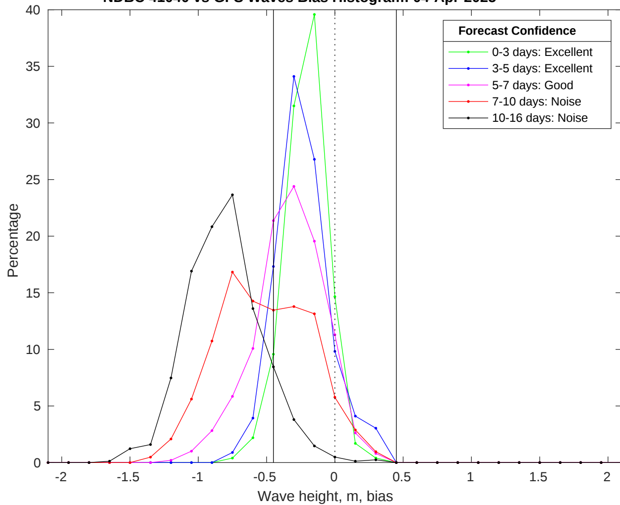
NDBC 41040 vs GFS Waves Bias Histogram: 04-Apr-2025
