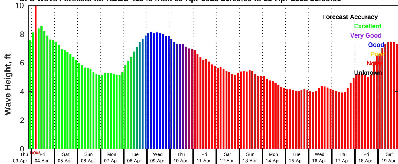
GFS Wave Forecast for NDBC 41040 from 03-Apr-2025 21:00:00 to 19-Apr-2025 21:00:00
