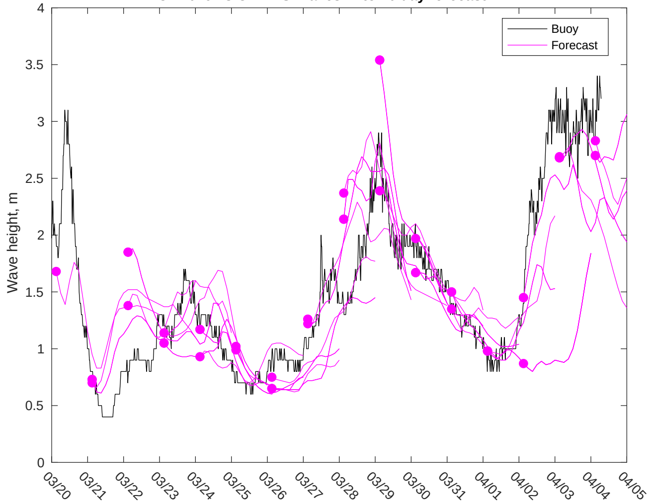
NDBC 42019 vs CMEMS Waves: 7 to 10 day forecast
