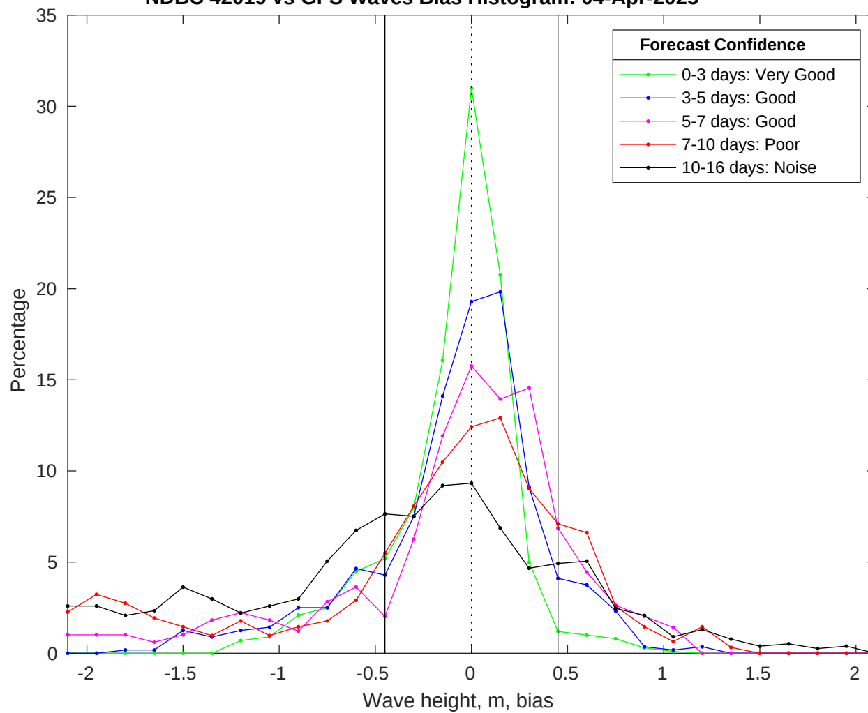
NDBC 42019 vs GFS Waves Bias Histogram: 04-Apr-2025
