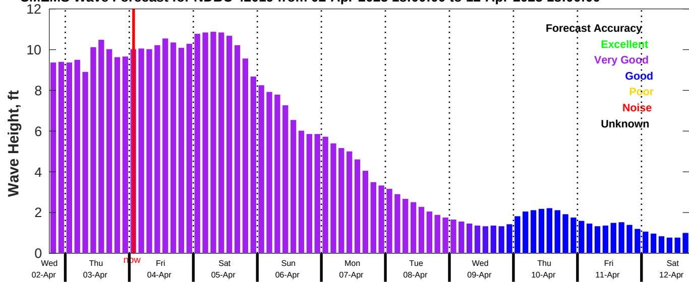
CMEMS Wave Forecast for NDBC 42019 from 02-Apr-2025 18:00:00 to 12-Apr-2025 18:00:00
