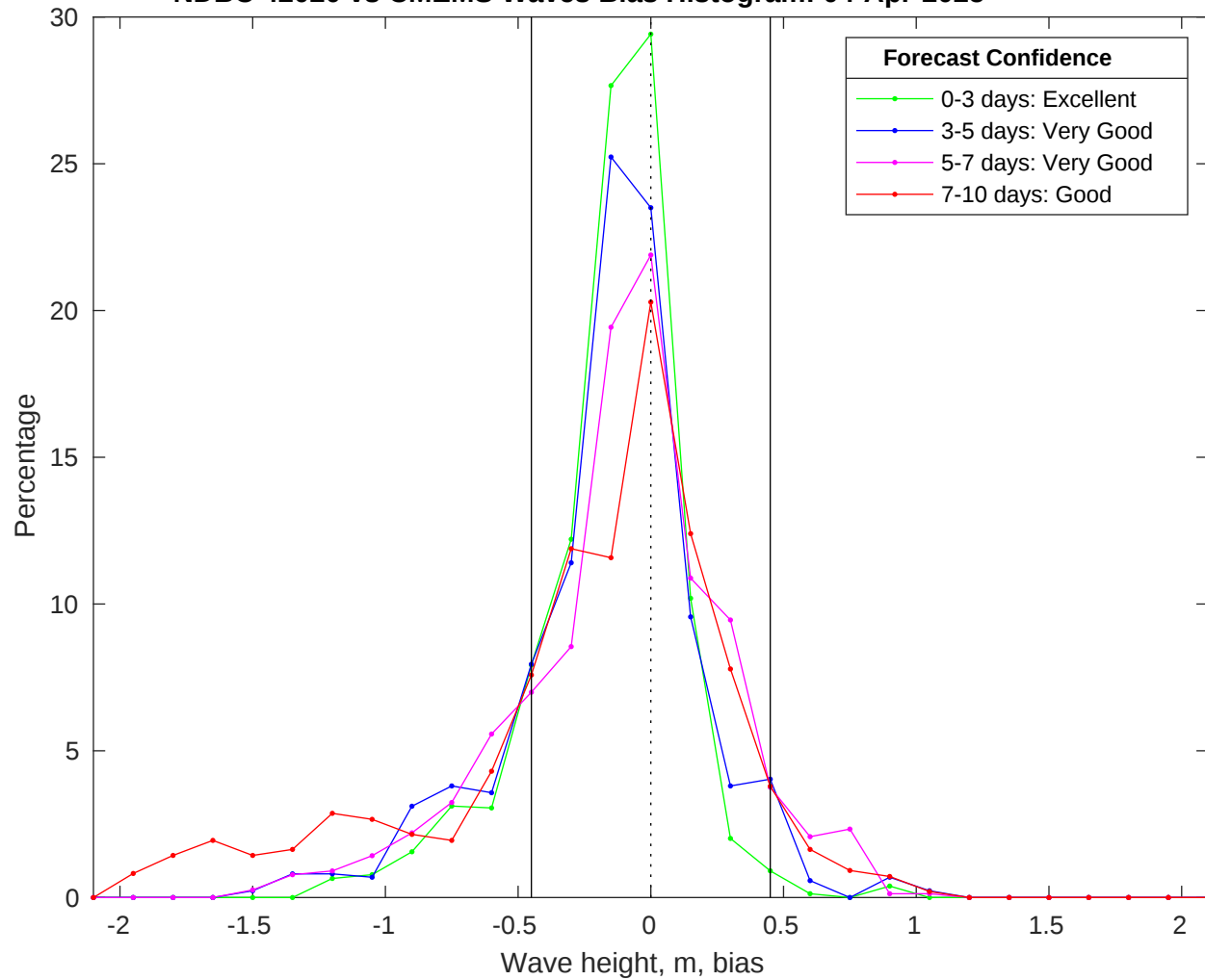
NDBC 42020 vs CMEMS Waves Bias Histogram: 04-Apr-2025
