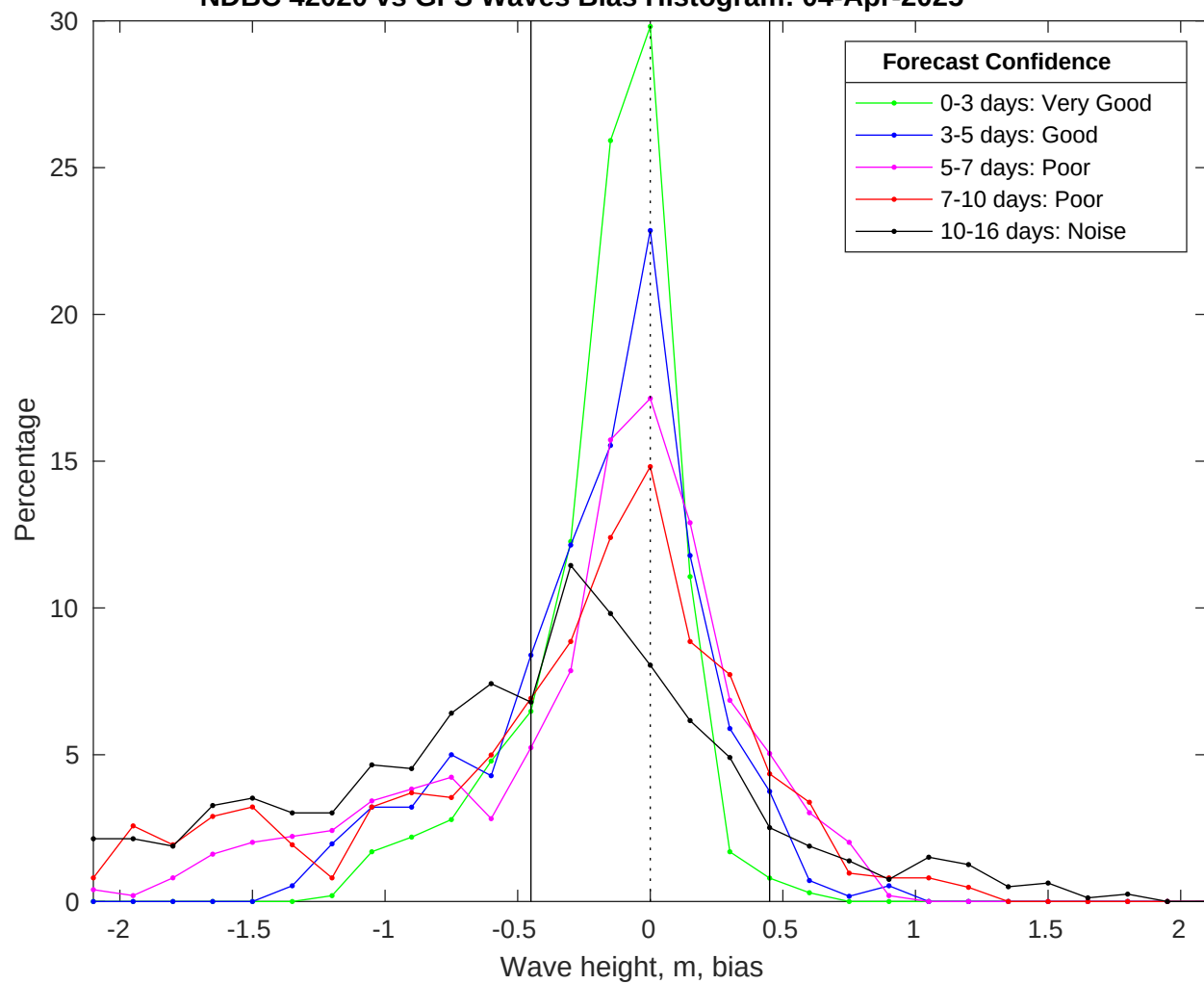
NDBC 42020 vs GFS Waves Bias Histogram: 04-Apr-2025
