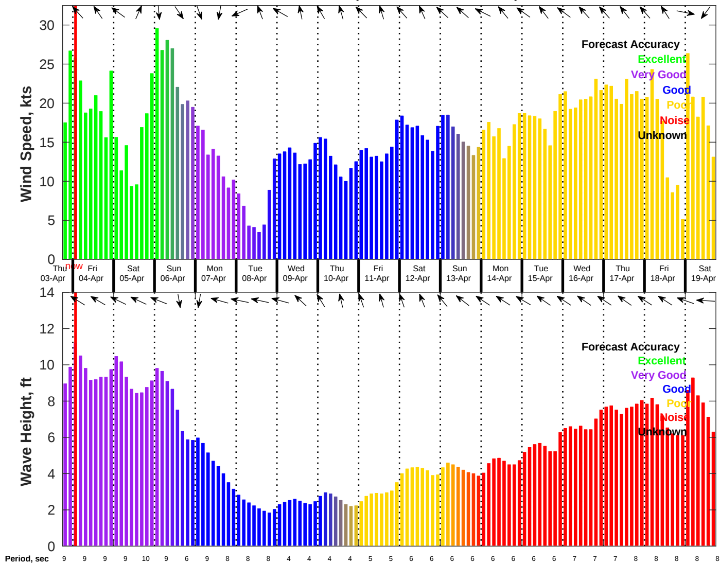
Wind & Wave Forecast for NDBC 42020 from 03-Apr-2025 18:00:00 to 19-Apr-2025 18:00:00
