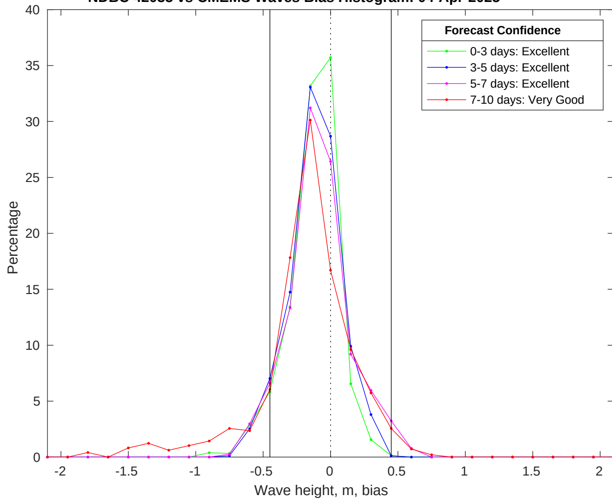
NDBC 42035 vs CMEMS Waves Bias Histogram: 04-Apr-2025
