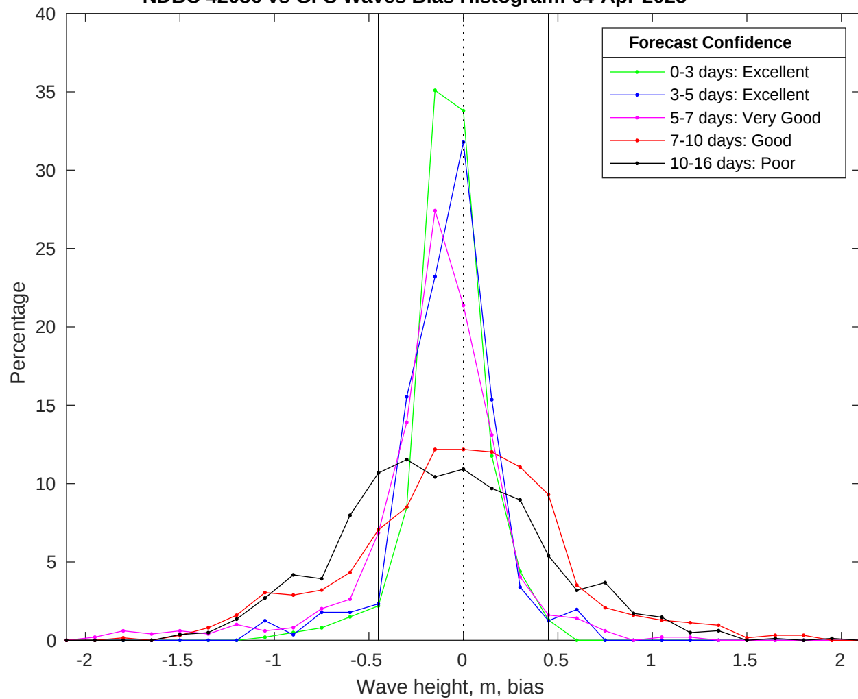
NDBC 42036 vs GFS Waves Bias Histogram: 04-Apr-2025
