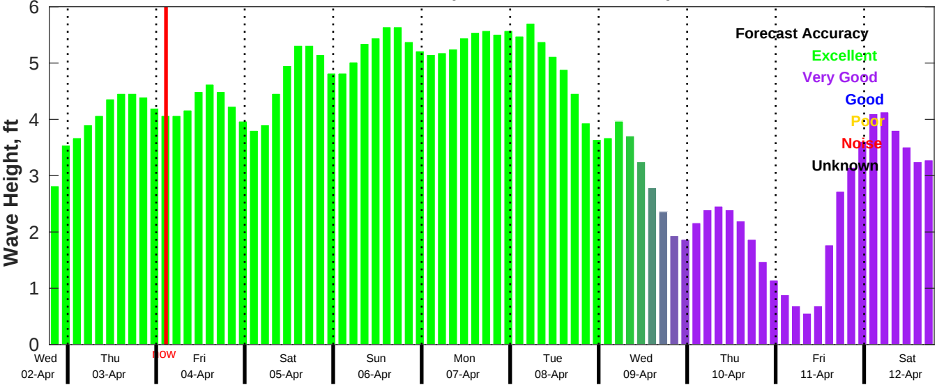
CMEMS Wave Forecast for NDBC 42036 from 02-Apr-2025 19:00:00 to 12-Apr-2025 19:00:00
