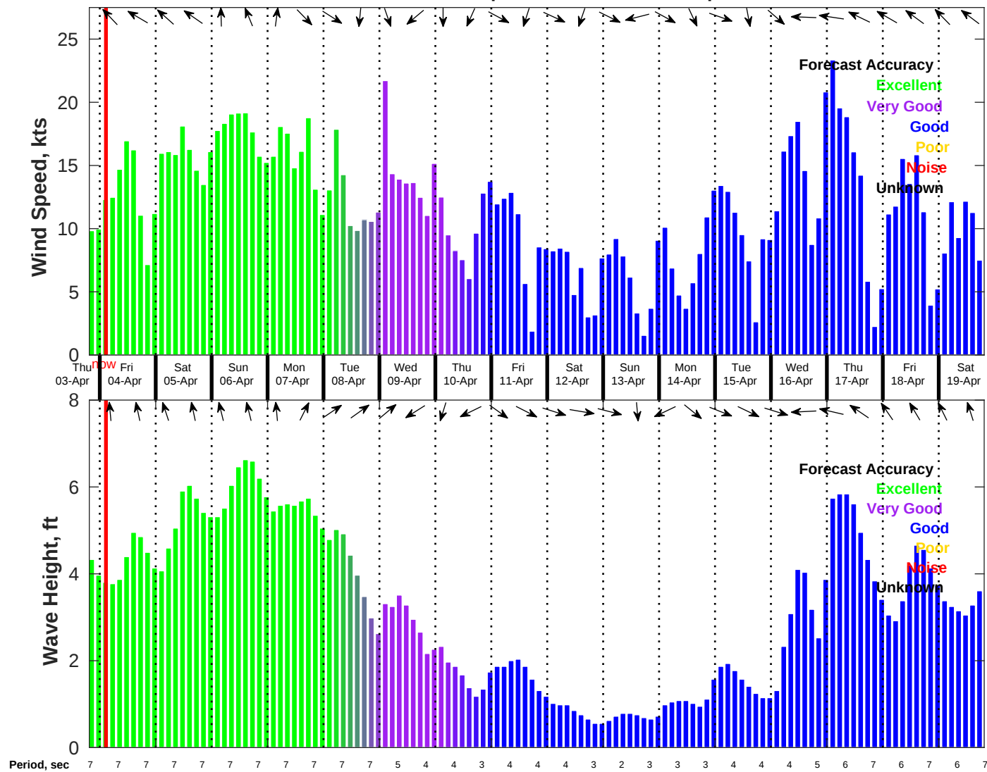
Wind & Wave Forecast for NDBC 42036 from 03-Apr-2025 19:00:00 to 19-Apr-2025 19:00:00
