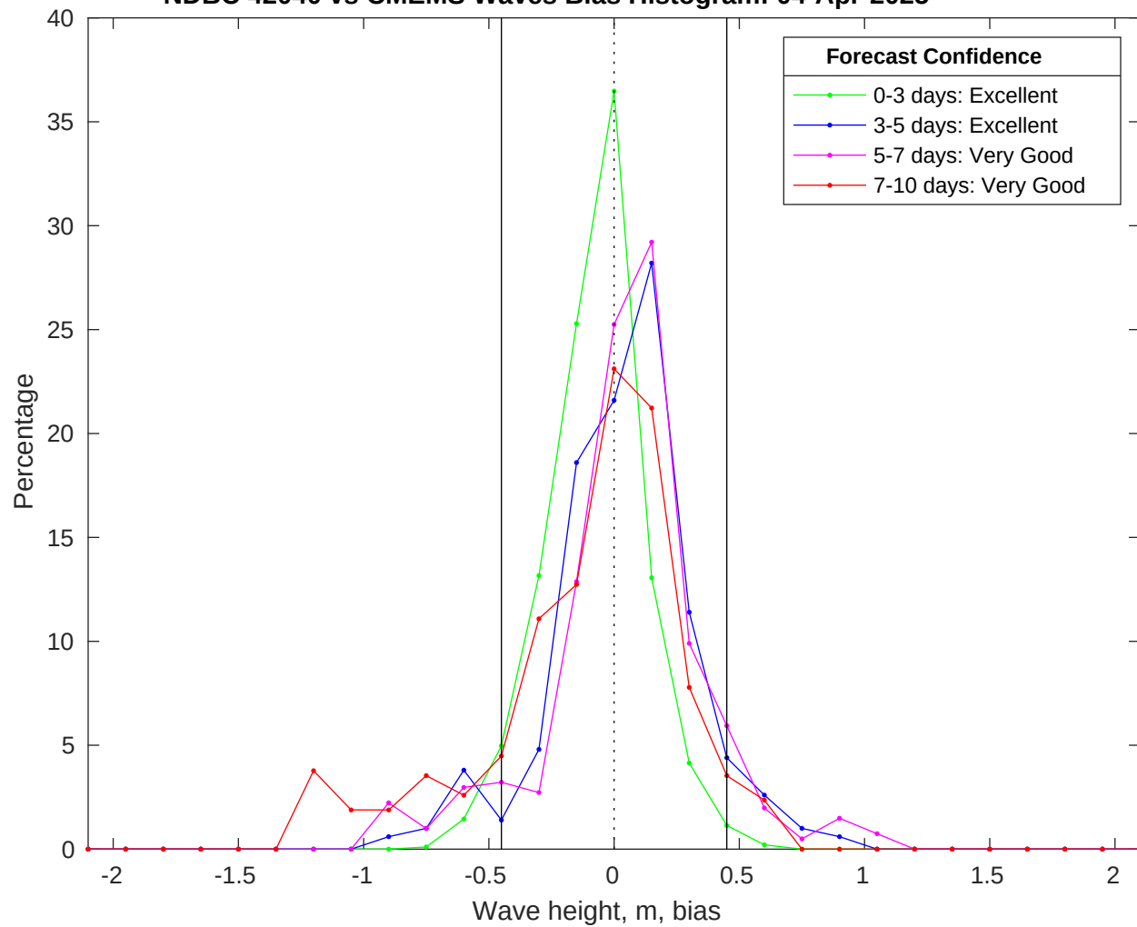
NDBC 42040 vs CMEMS Waves Bias Histogram: 04-Apr-2025
