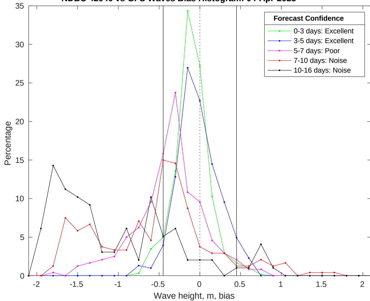
NDBC 42040 vs GFS Waves Bias Histogram: 04-Apr-2025
