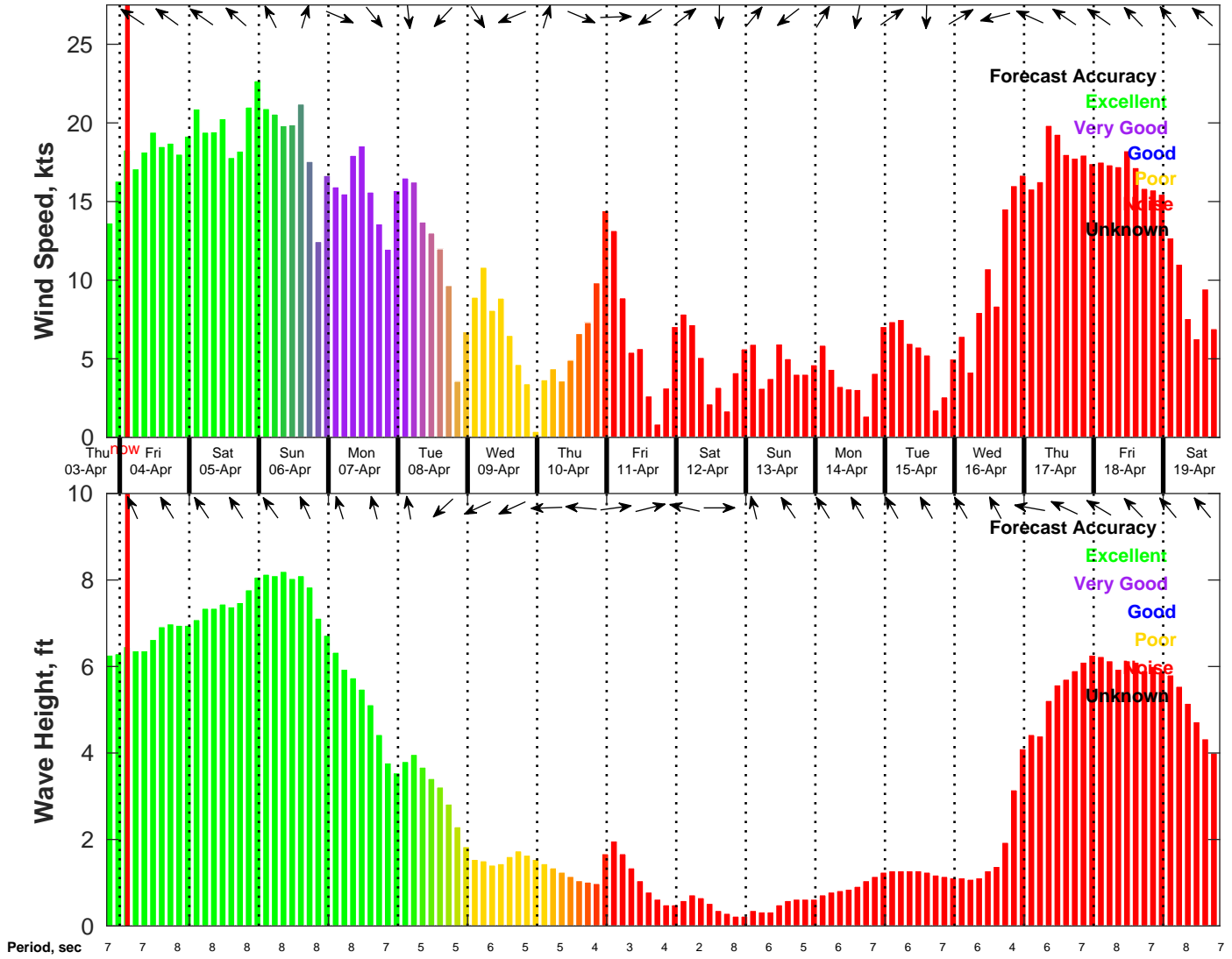
Wind & Wave Forecast for NDBC 42040 from 03-Apr-2025 19:00:00 to 19-Apr-2025 19:00:00
