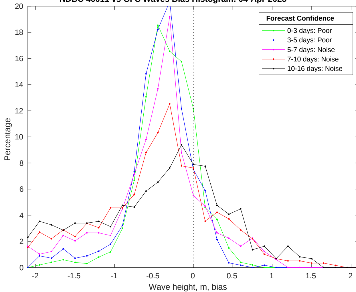
NDBC 46011 vs GFS Waves Bias Histogram: 04-Apr-2025
