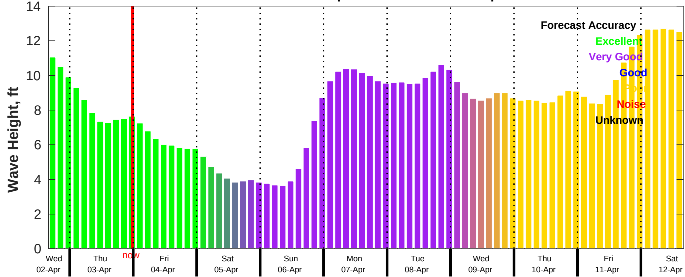
CMEMS Wave Forecast for NDBC 46011 from 02-Apr-2025 16:00:00 to 12-Apr-2025 16:00:00
