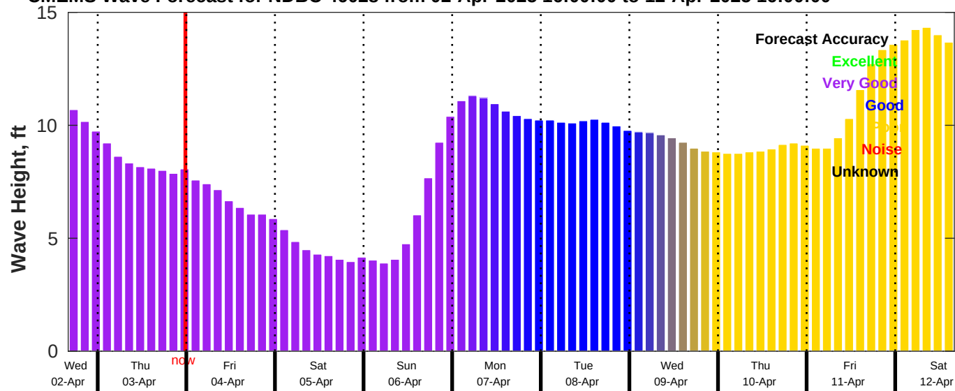
CMEMS Wave Forecast for NDBC 46028 from 02-Apr-2025 16:00:00 to 12-Apr-2025 16:00:00
