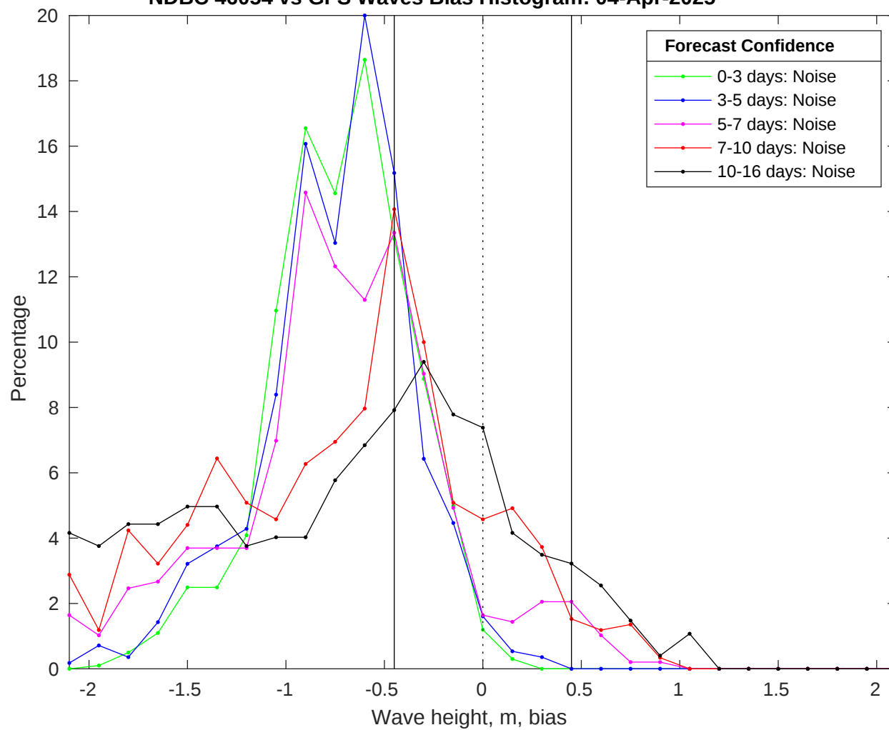
NDBC 46054 vs GFS Waves Bias Histogram: 04-Apr-2025
