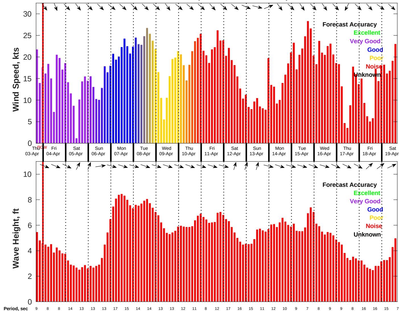
Wind & Wave Forecast for NDBC 46054 from 03-Apr-2025 16:00:00 to 19-Apr-2025 16:00:00
