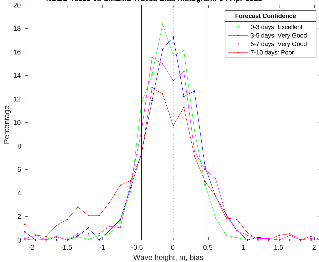
NDBC 46069 vs CMEMS Waves Bias Histogram: 04-Apr-2025
