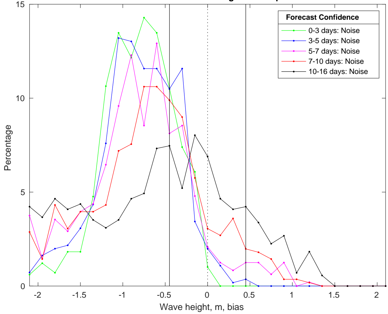
NDBC 46069 vs GFS Waves Bias Histogram: 04-Apr-2025
