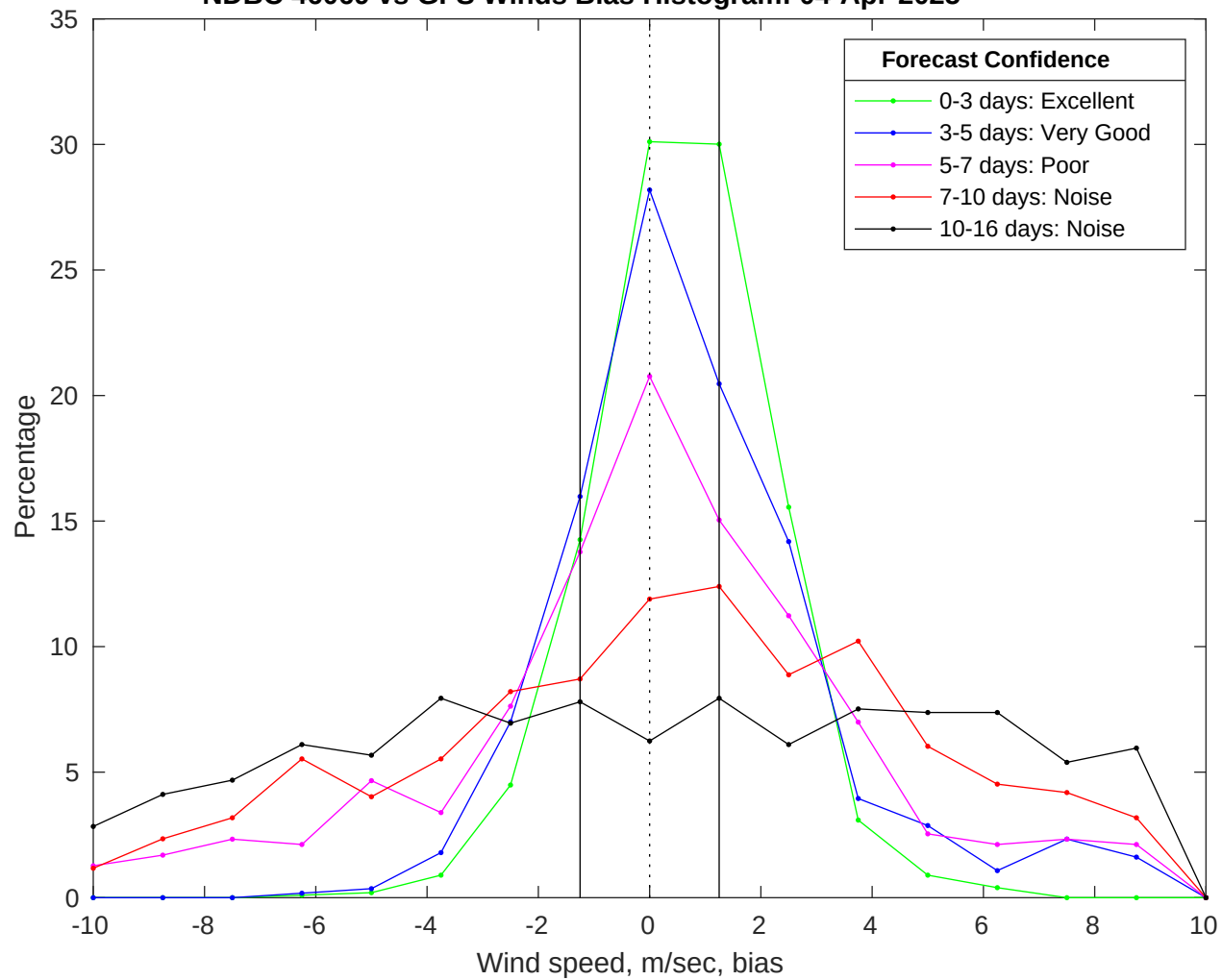
NDBC 46069 vs GFS Winds Bias Histogram: 04-Apr-2025
