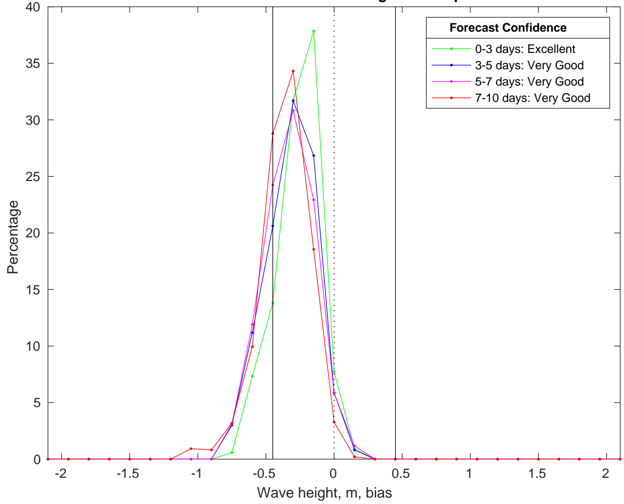
NDBC 51209 vs CMEMS Waves Bias Histogram: 04-Apr-2025
