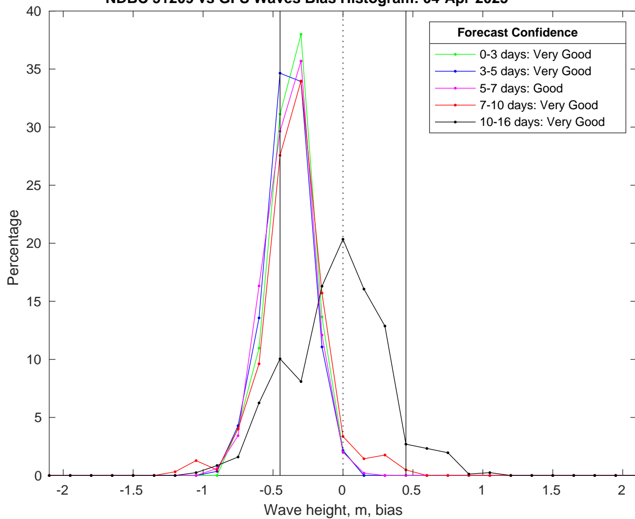
NDBC 51209 vs GFS Waves Bias Histogram: 04-Apr-2025
