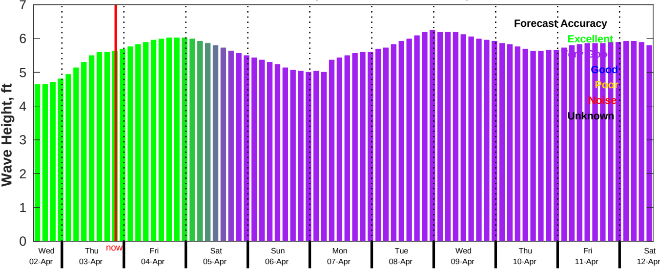
CMEMS Wave Forecast for NDBC 51209 from 02-Apr-2025 13:00:00 to 12-Apr-2025 13:00:00
