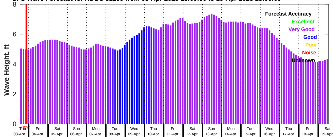
GFS Wave Forecast for NDBC 51209 from 03-Apr-2025 13:00:00 to 19-Apr-2025 13:00:00
