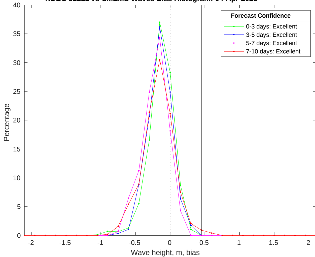
NDBC 52211 vs CMEMS Waves Bias Histogram: 04-Apr-2025
