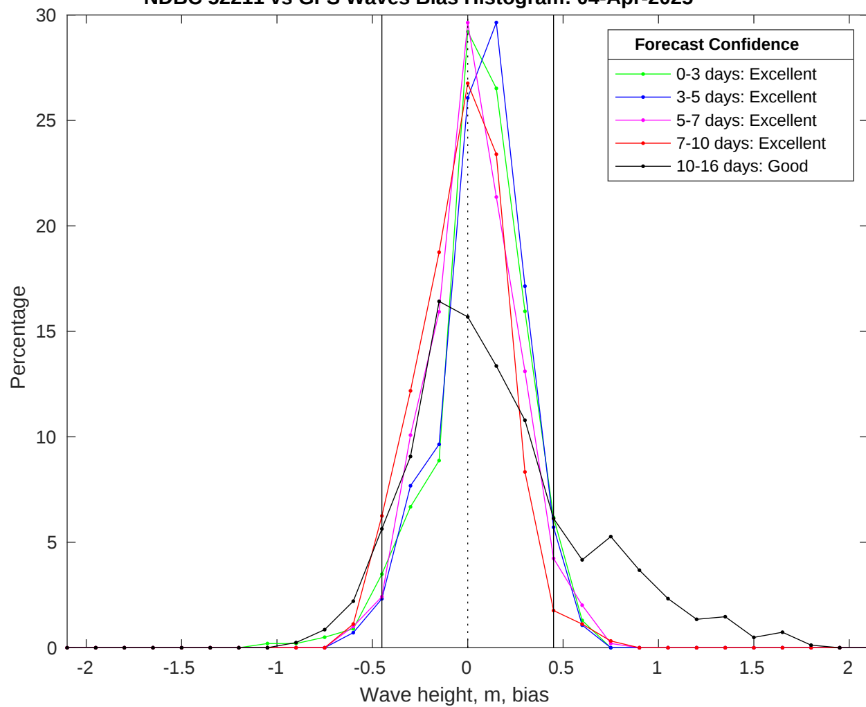
NDBC 52211 vs GFS Waves Bias Histogram: 04-Apr-2025
