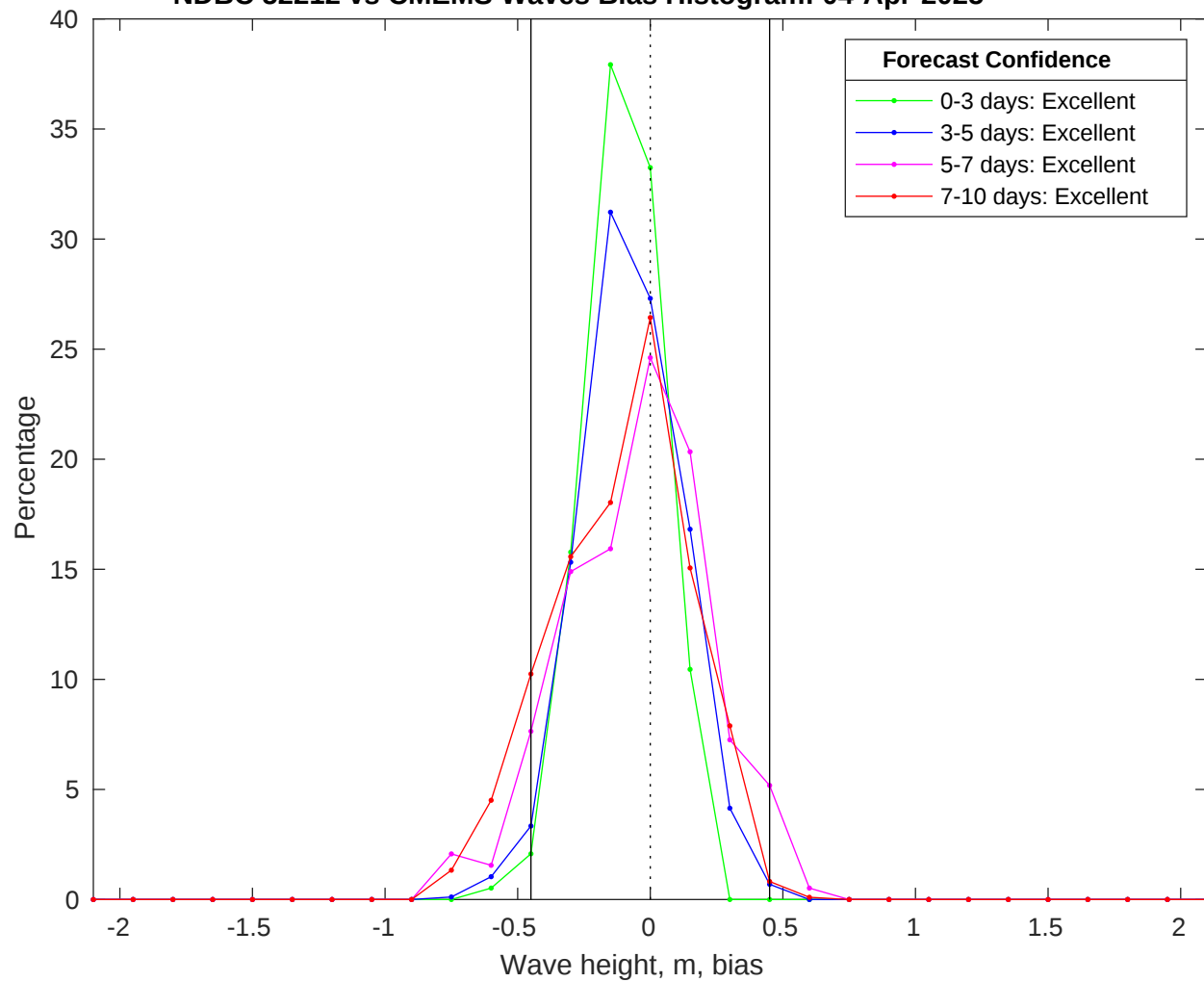
NDBC 52212 vs CMEMS Waves Bias Histogram: 04-Apr-2025
