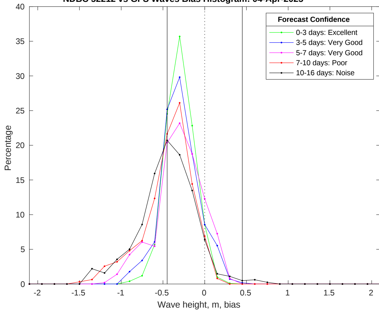
NDBC 52212 vs GFS Waves Bias Histogram: 04-Apr-2025
