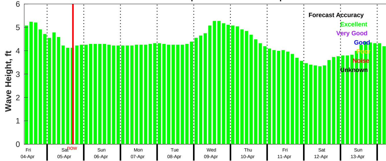
CMEMS Wave Forecast for NDBC 52212 from 03-Apr-2025 09:00:00 to 13-Apr-2025 09:00:00
