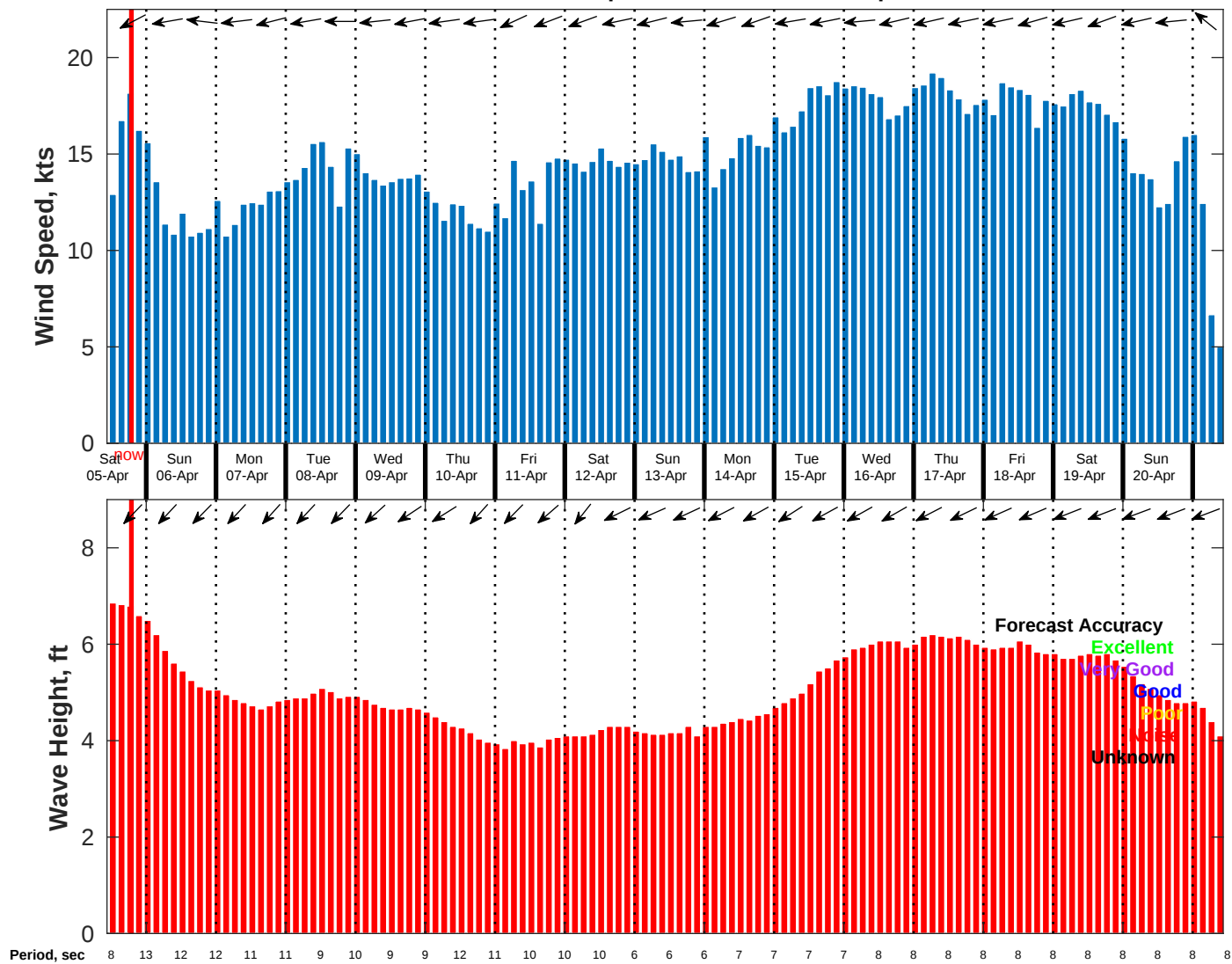
Wind & Wave Forecast for NDBC 52213 from 04-Apr-2025 11:00:00 to 20-Apr-2025 11:00:00
